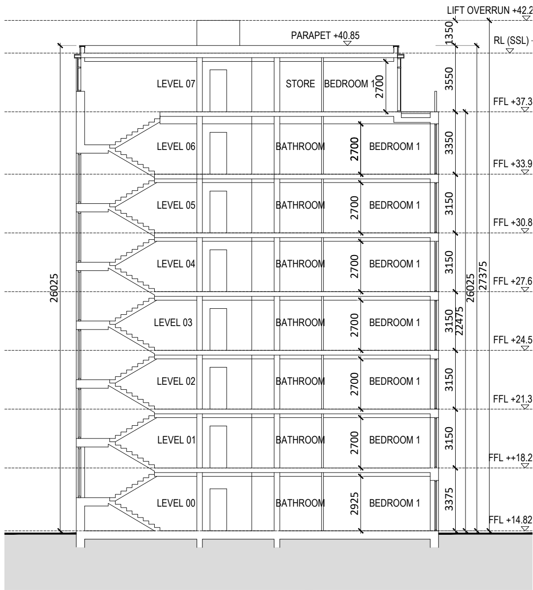
SECTION AA
