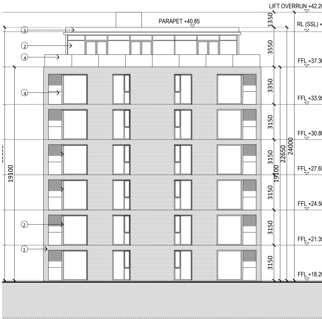
SOUTH ELEVATION
