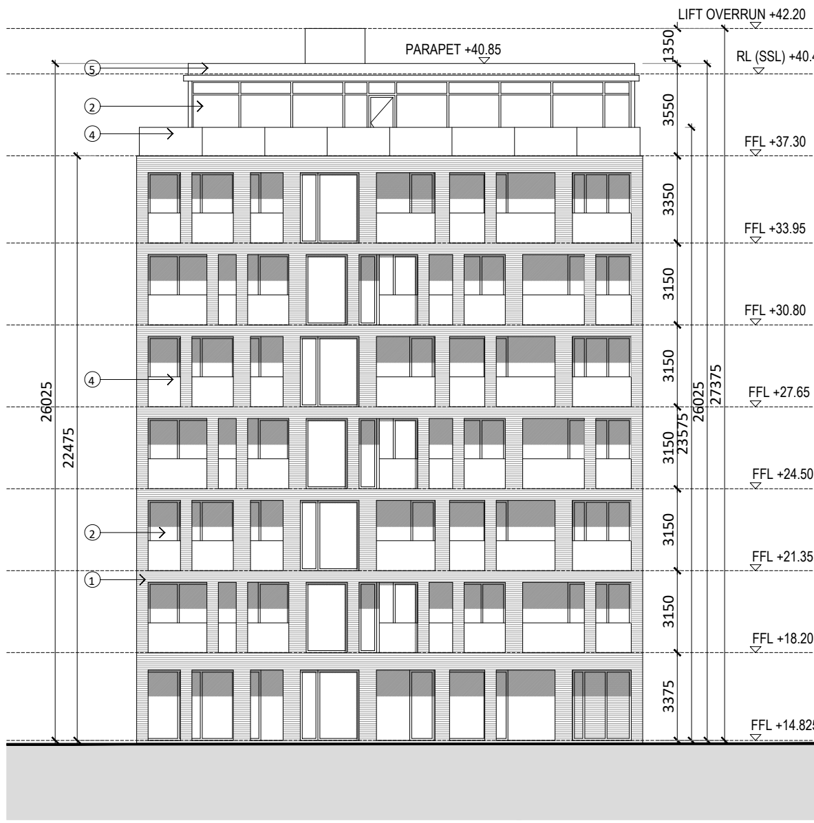
NORTH ELEVATION
